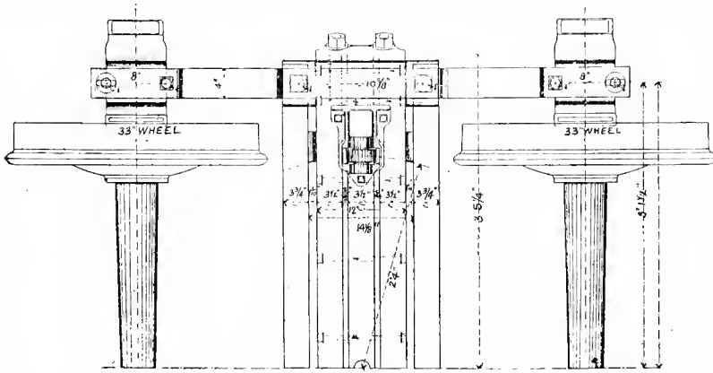
Fig. 4747. Half Plan.
